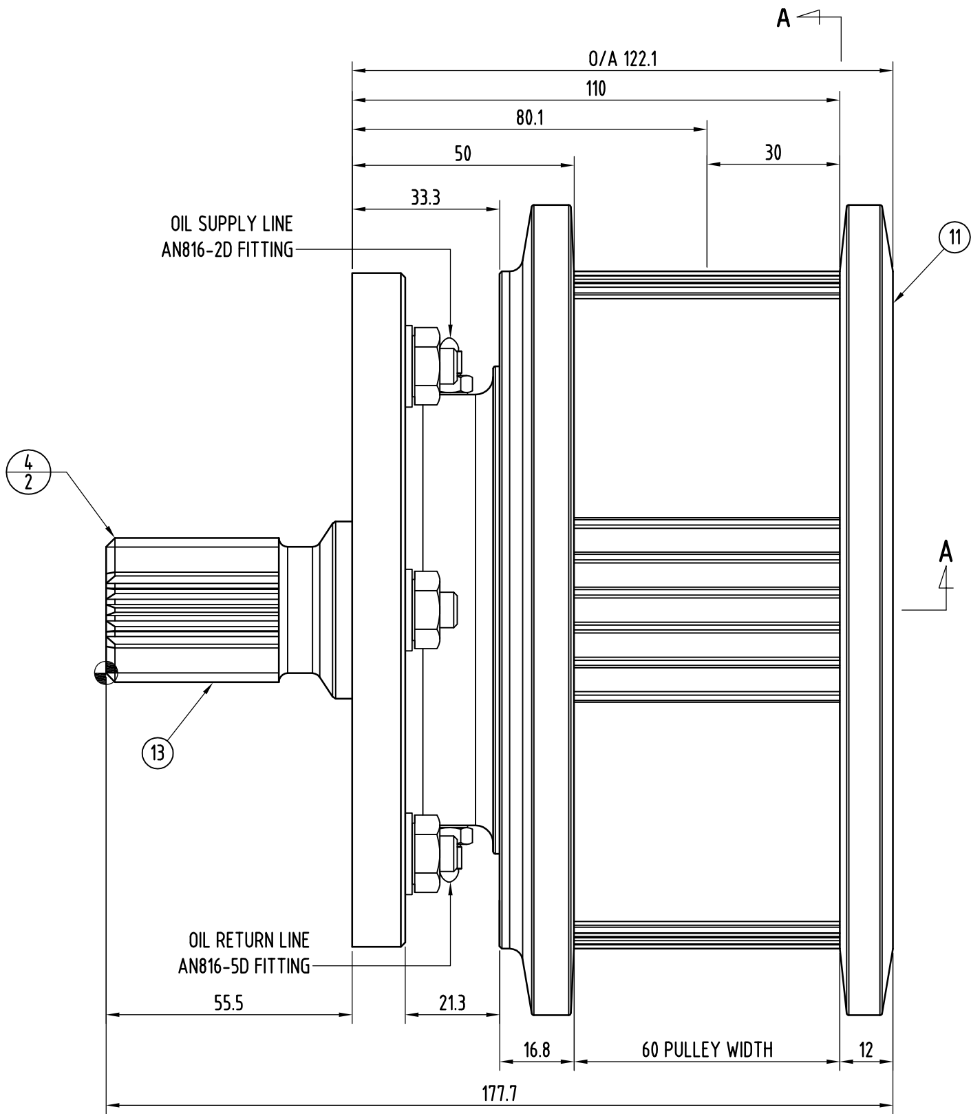
PLAN VIEW
